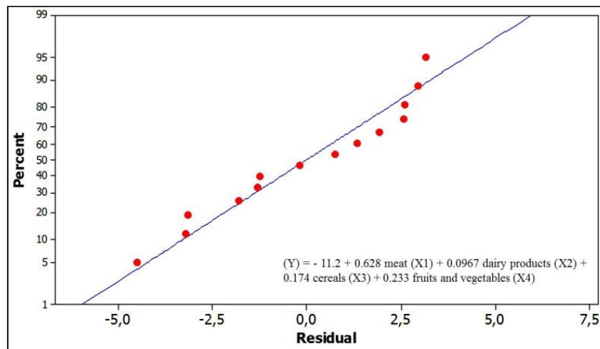
Fig. 1. Multiple linear regression graph for world food prices in dollars (US$)
