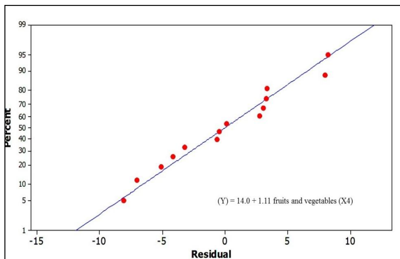
Fig. 4. Simple linear regression graph of the price of fruits and vegetables (X 4 ) in Brazil in reals (R$)
