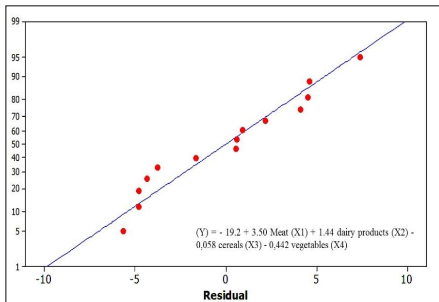
Fig. 2. Multiple linear regression graph for food prices in Brazil in reals (R$)
