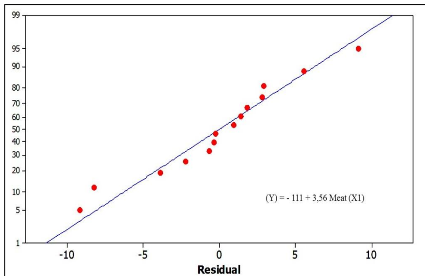
Fig. 3. Simple linear regression graph of meat price ( X_1 ) in Brazil in reais (R$)
