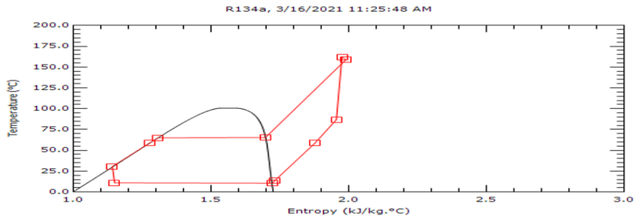
Fig. 4. Simulation analysis of R134A refrigerants
