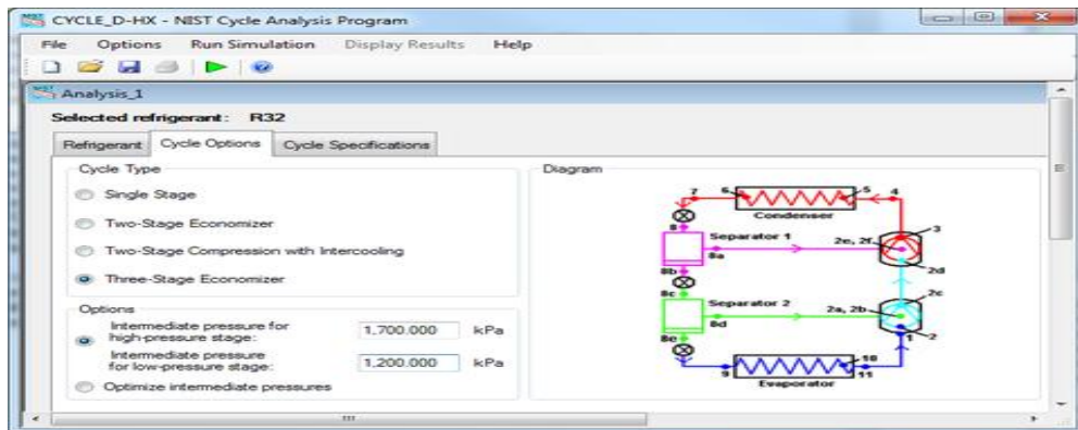
Fig. 2. CYCLE_D-HX simulator
