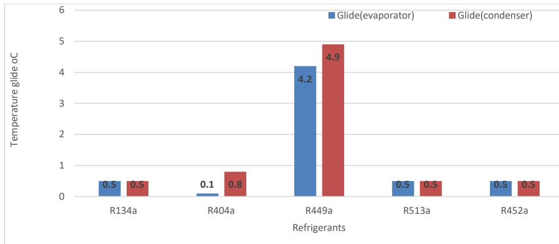
Fig. 12. Temperature glide in the evaporator and condenser for each refrigerant
