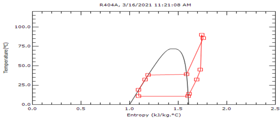
Fig. 5. Simulation analysis of R404A refrigerants
