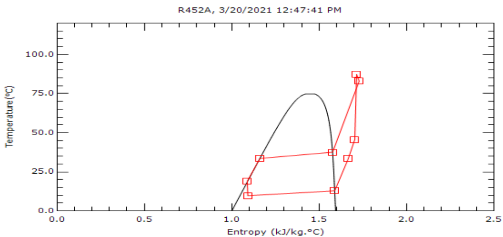
Fig. 8. Simulation analysis of R452A refrigerants
