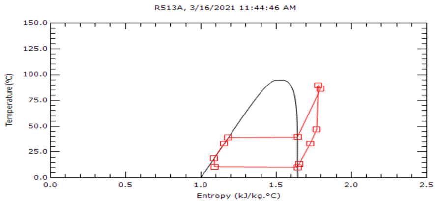
Fig. 7. Simulation analysis of R513A refrigerants
