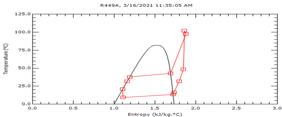
Fig. 6. Simulation analysis of R449A refrigerants
