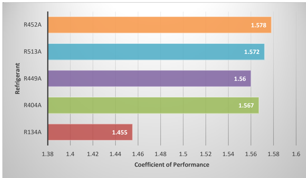
Fig. 9. Coefficient of performance of the refrigerants
