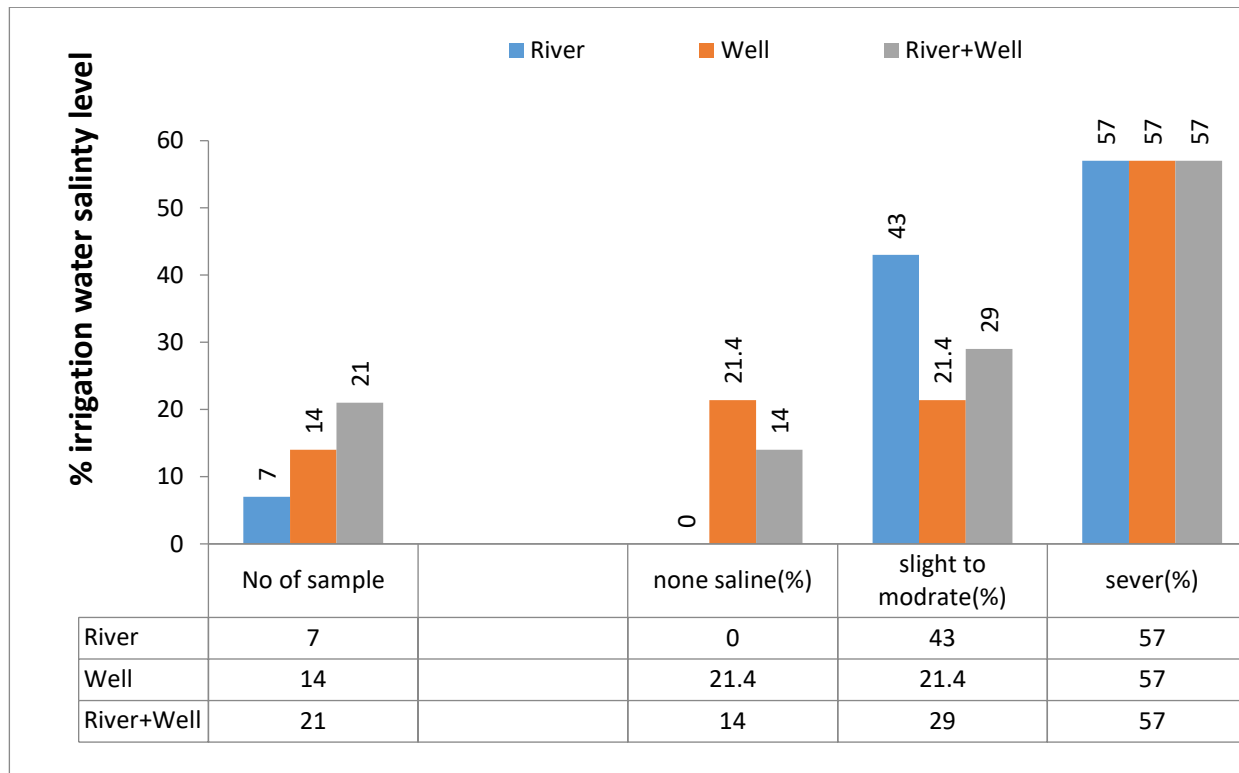
Fig. 3. Status of water quality at mentebteb at farmer level irrigation site
