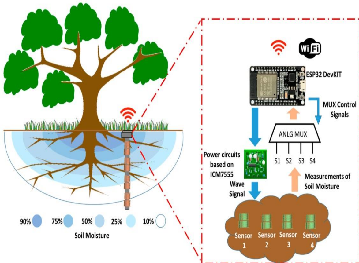
Fig. 1. Schematic representation of a nanotechnology-enabled wireless sensor network for soil monitoring in precision agriculture
