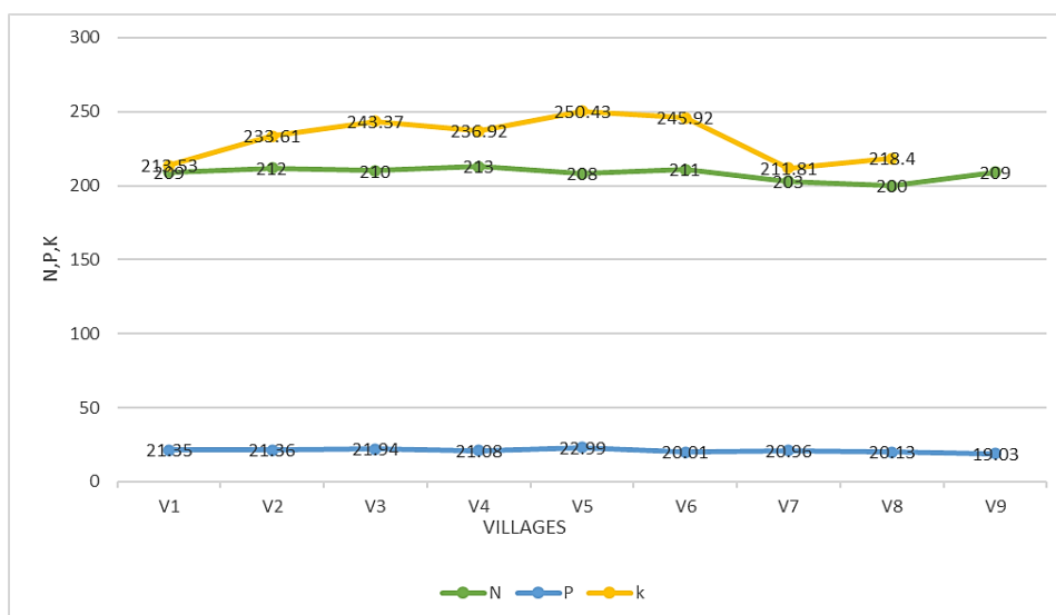
Fig. 5. Available nitrogen, phosphorous and potassium (Kg ha -1 )
