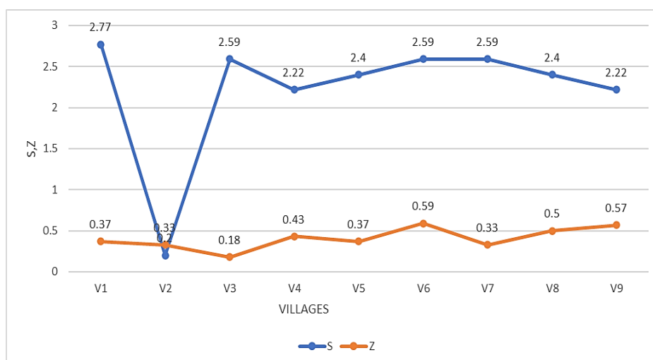
Fig. 6. sulphur(ppm) and zinc(ppm)
