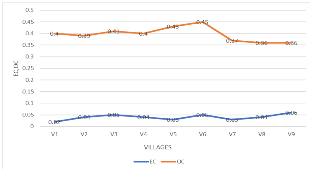
Fig. 4. EC (ds m -1 ) and OC (%)
