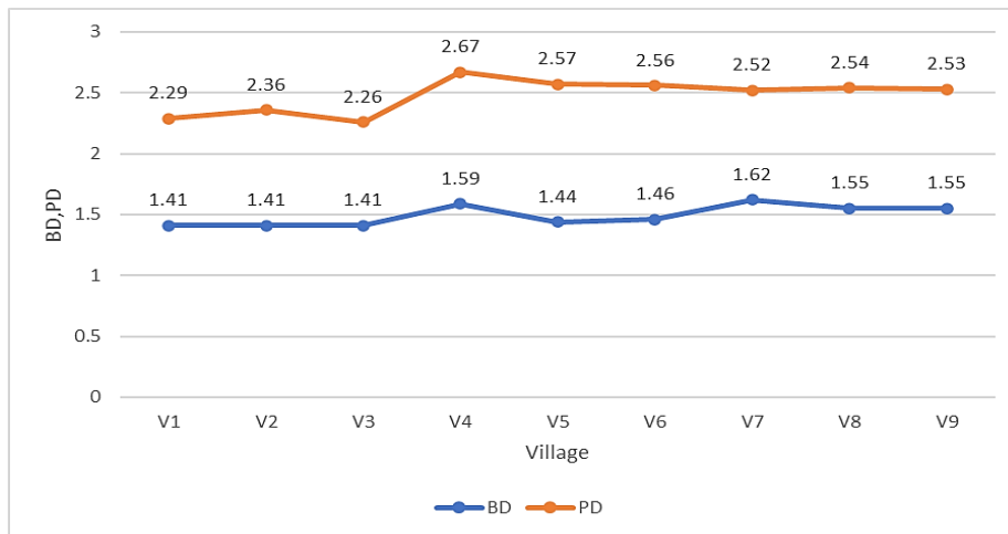
Fig. 1. Bulkdensity (Mg m -3 ) and partical density(Mg m -3 )
