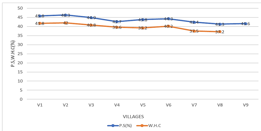
Fig. 2. Pore space(%) and water holding capacity(%)
