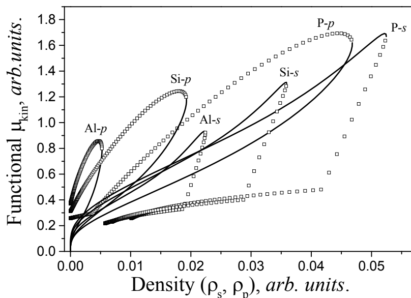
Fig. 3. Dependencies \mu_{kin}^s(\rho_s) and \mu_{kin}^p(\rho_p) for Al, Si, and P single atoms. Solid curves describe functionals in outside valence regions, the hole quadrates demonstrate behavior of functionals inside core spheres
