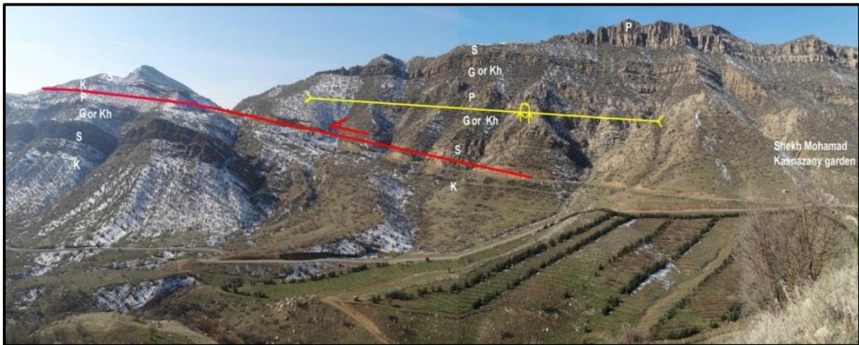
Figure 11. Inner arc of the southwestern limb of the Sagrma anticline along the road between Qaradagh and Sangaw towns, near the Garden of Shekh Mohamad Kasnazany shows the lateral thrust and overturned syncline
