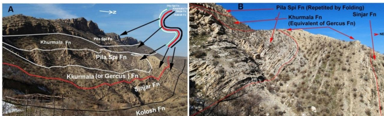
Figure 3. Stratigraphic differentiation of the inner arc of the southwestern limb Sagerma (Sagerma) anticline 1km to the Shekh Mohamad Kasanaziny garden. A) This photo shows the same view of the Lawa (2004, see the below photo). B) Close up of the repetition of the Pila Spi and Khurmala Formations
